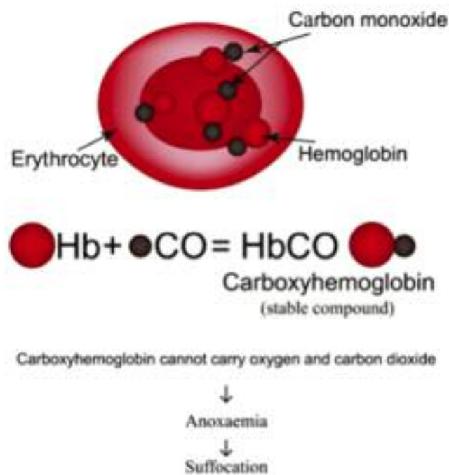
Fig. 1 - Carbon monoxide binding to hemoglobin.
